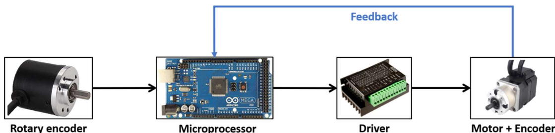
Figure 3: Single joint control mechanism showing the flowchart of ROM signal processing for motor control.
