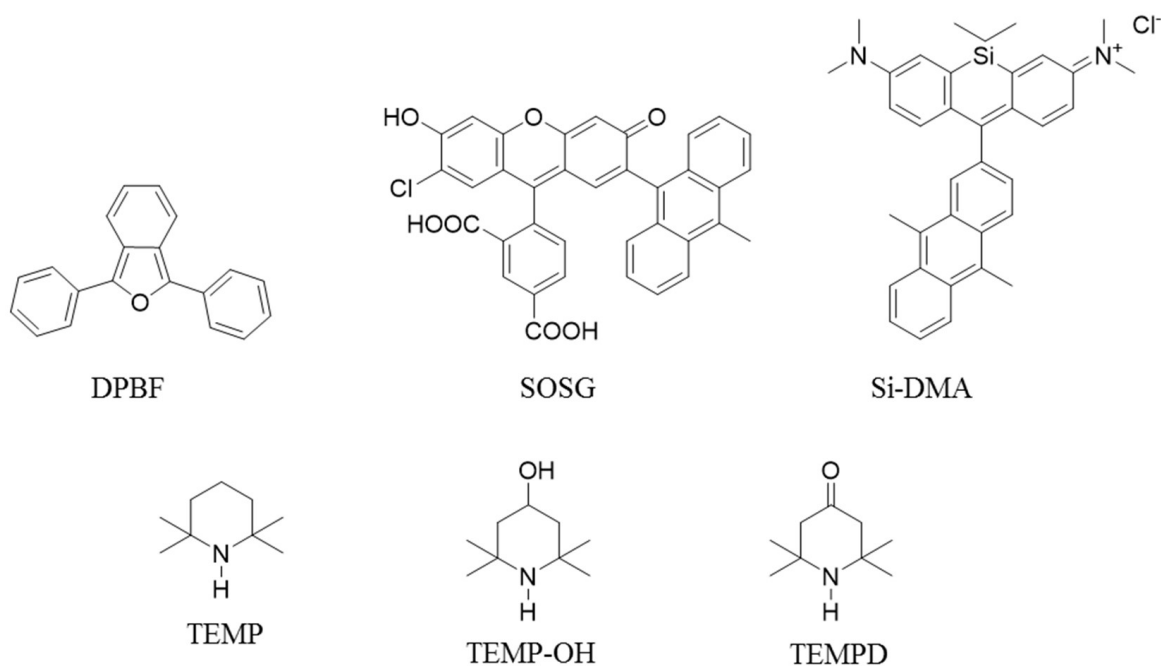
Figure 1: Chemical structure of detector probes.
